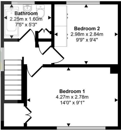
First Floor Approx 31 sq m / 333 sq ft
